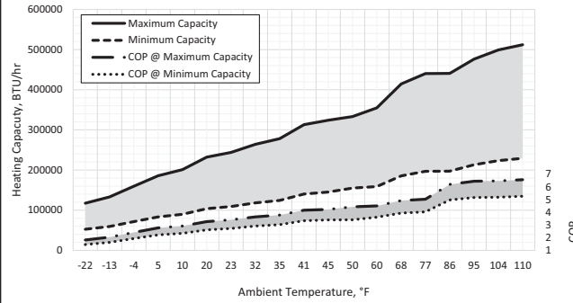
110°F Leaving Water Temperature, Heating
