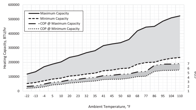
100°F Leaving Water Temperature, Heating
