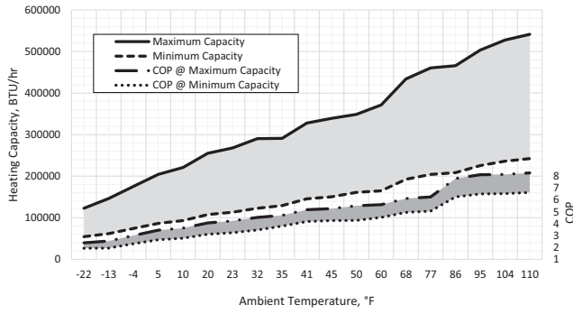
80°F Leaving Water Temperature, Heating
