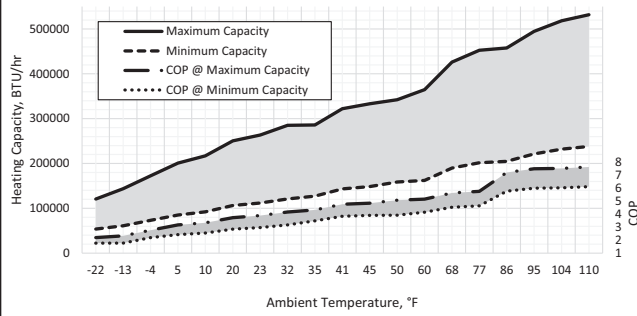
90°F Leaving Water Temperature, Heating
